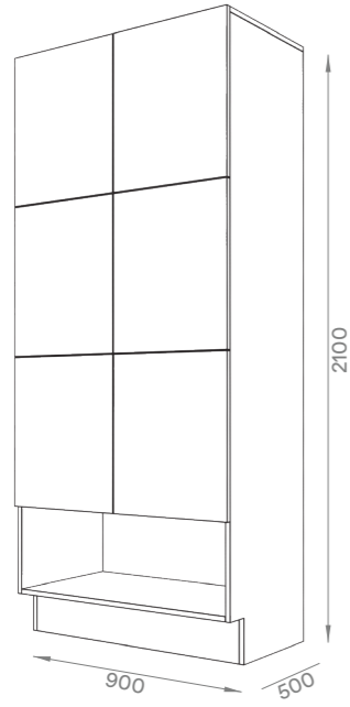
3-Tier double open bay 150mm toekick 300mm open bay
