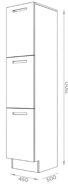
3-Tier with mail slot 150mm toekick
