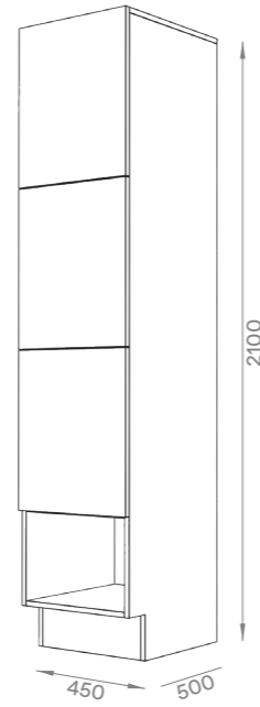
3-Tier open bay 150mm toekick 300mm open bay
